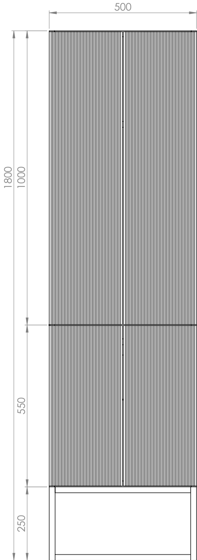
Front View
