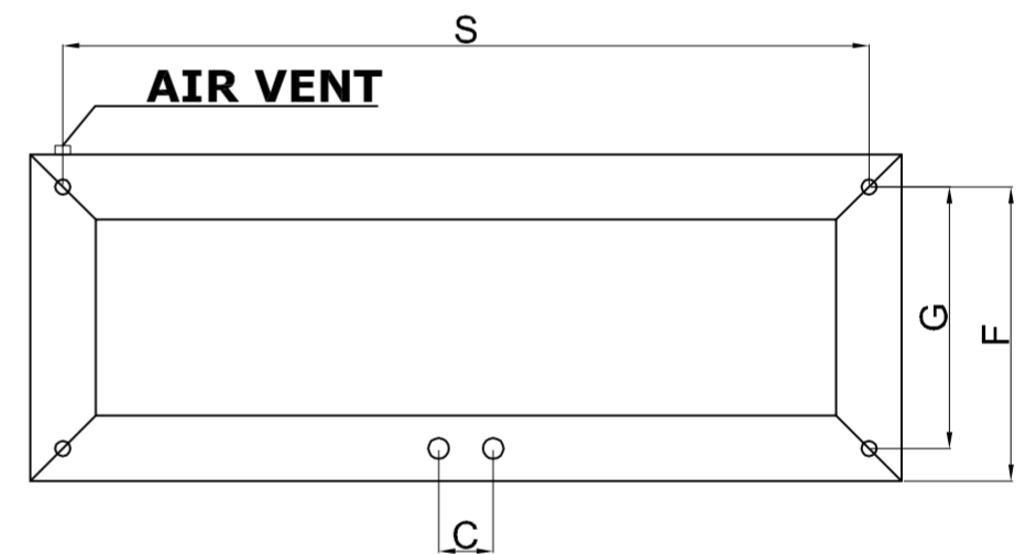
Back View
