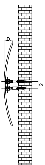
Top View
