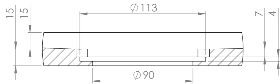
DETAIL B SCALE 1 : 2
