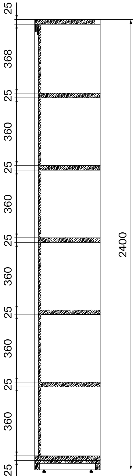
Side View
