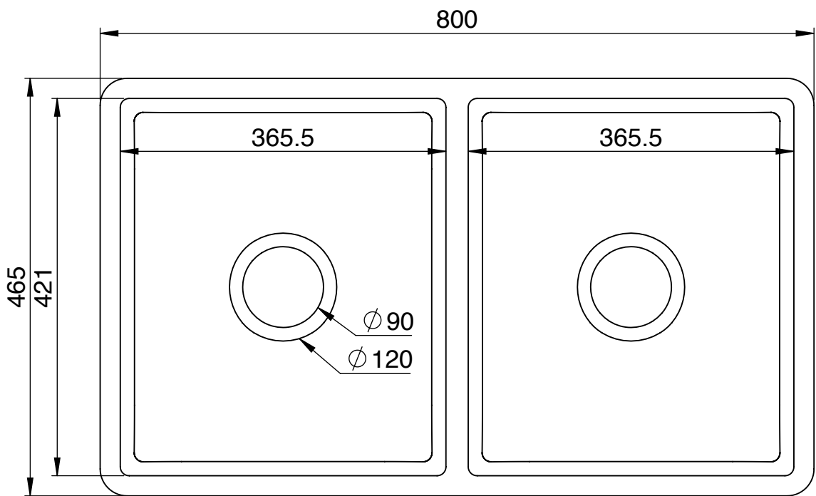
Top View
