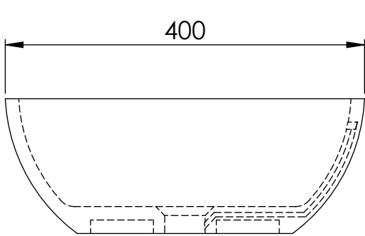
Side View - Section View
