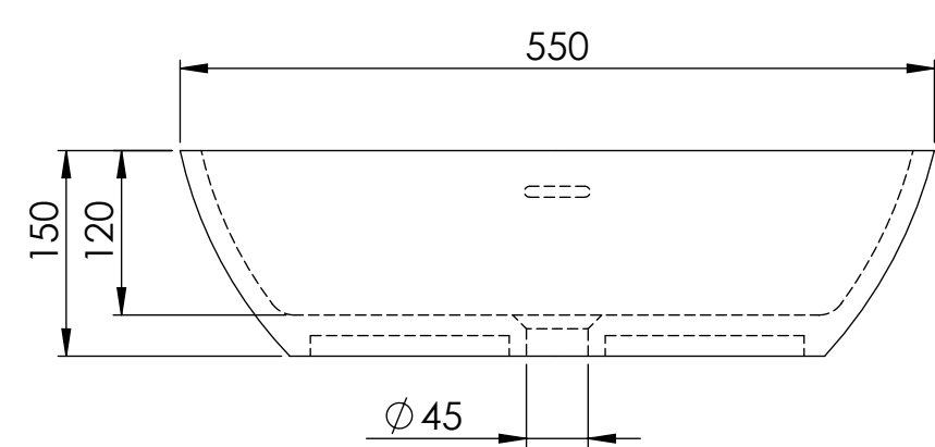
Front View - Section View
