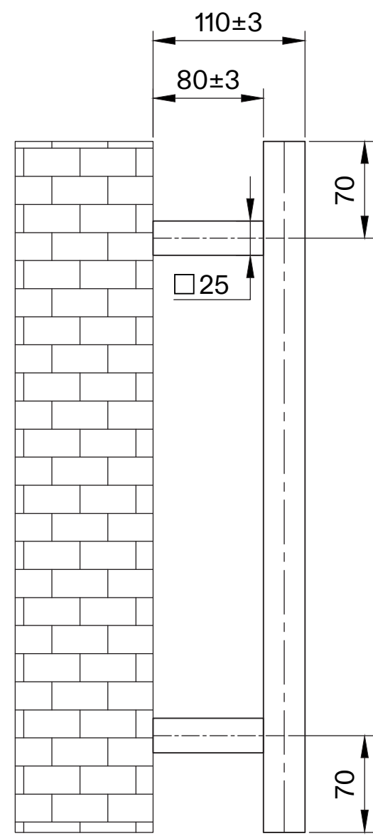
Side View
