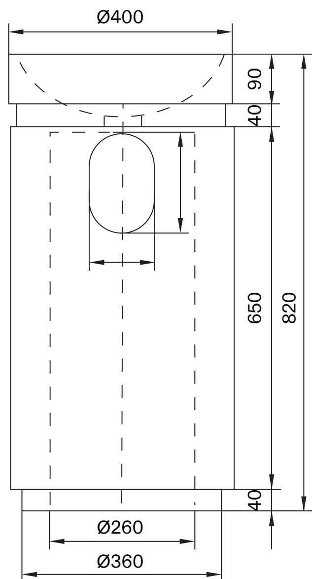
Back View - Section View
