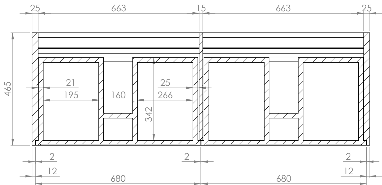
Top View - Section View
