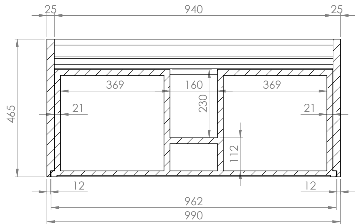
Top View - Section View
