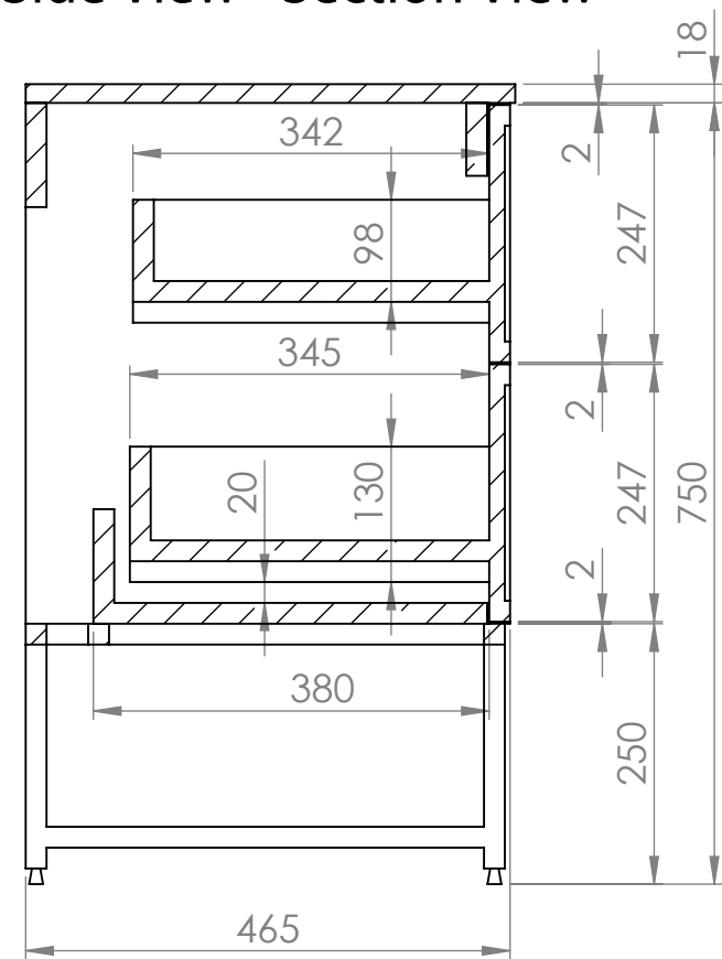
Side View - Section View
