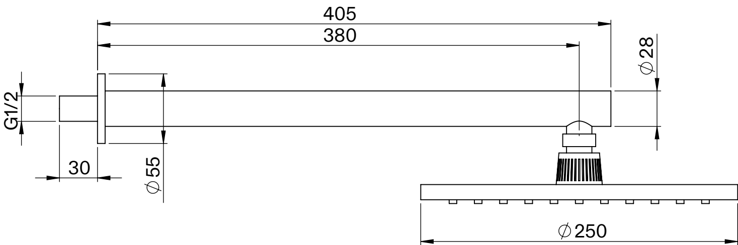
Side View - Shower
