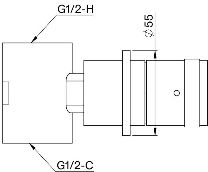
Top View - Valve
