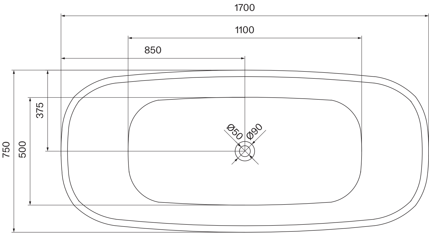
Top View
