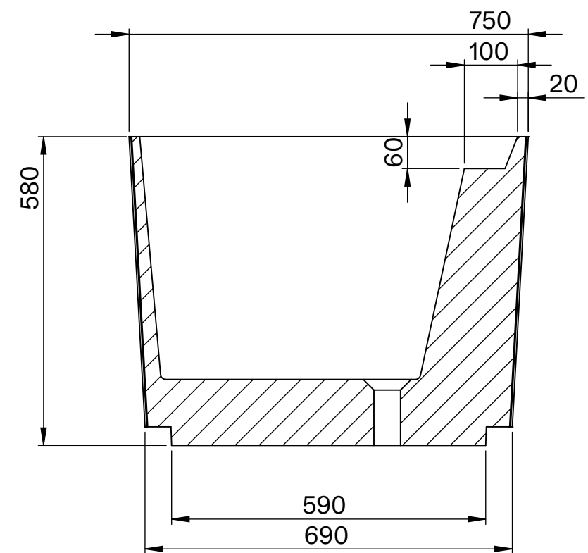
Side View - Section View
