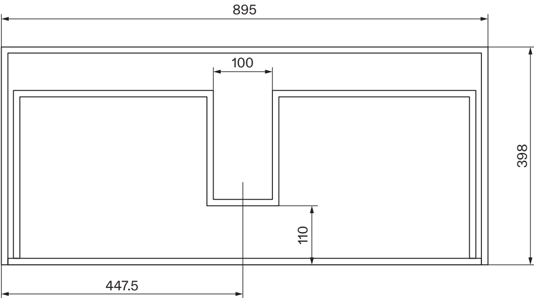
Top View Draw - Section View
