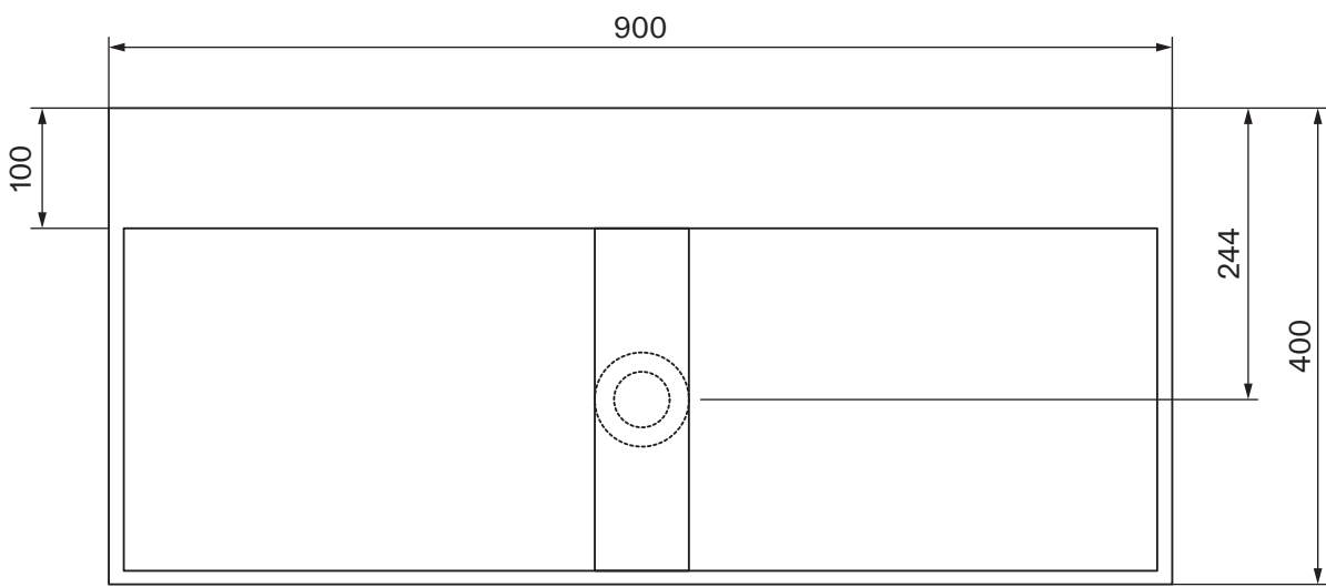
Top View - Basin
