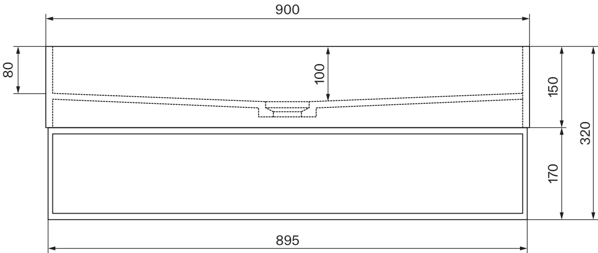
Front View - Section View
