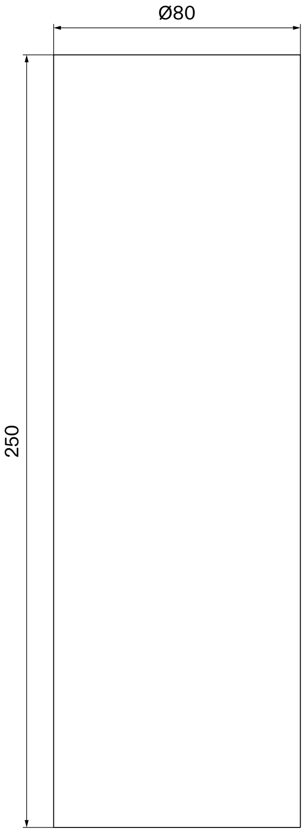
Front View
