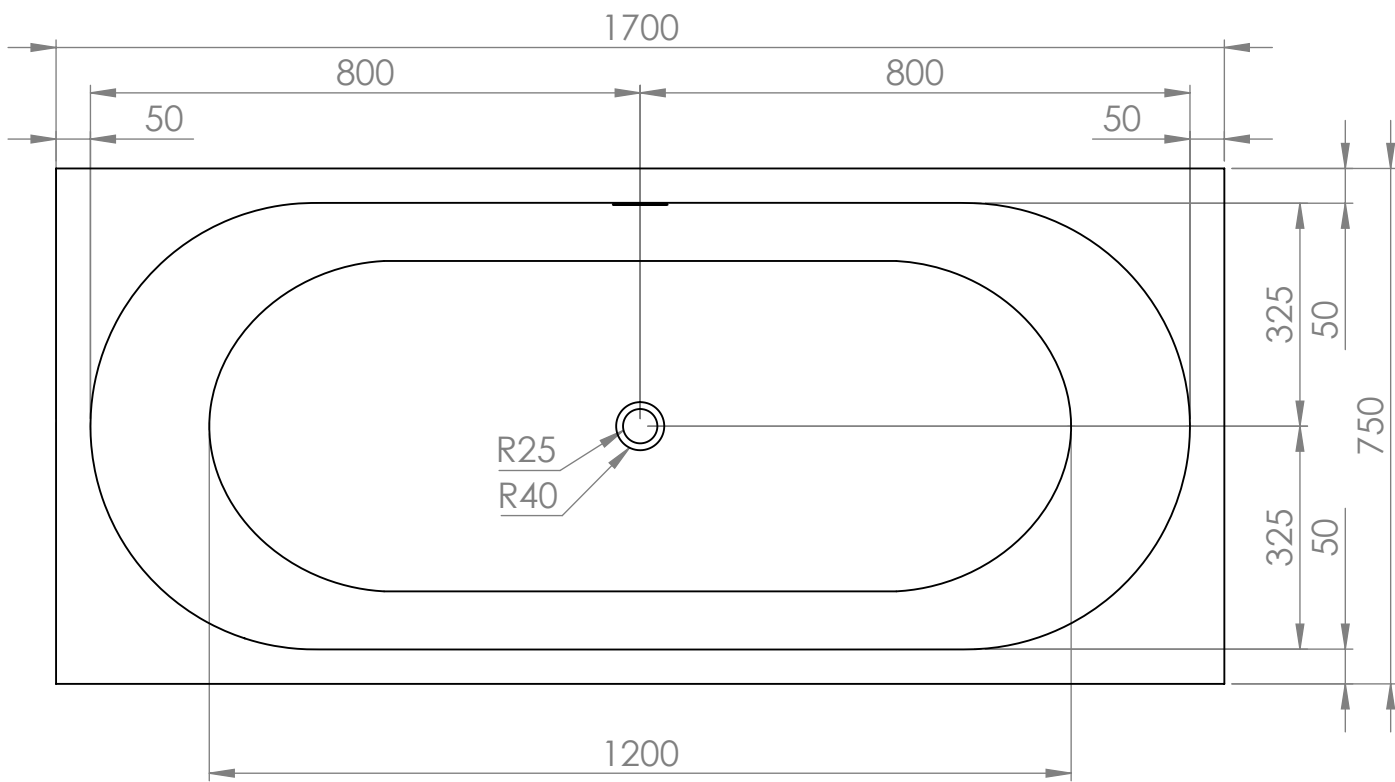
Top View
