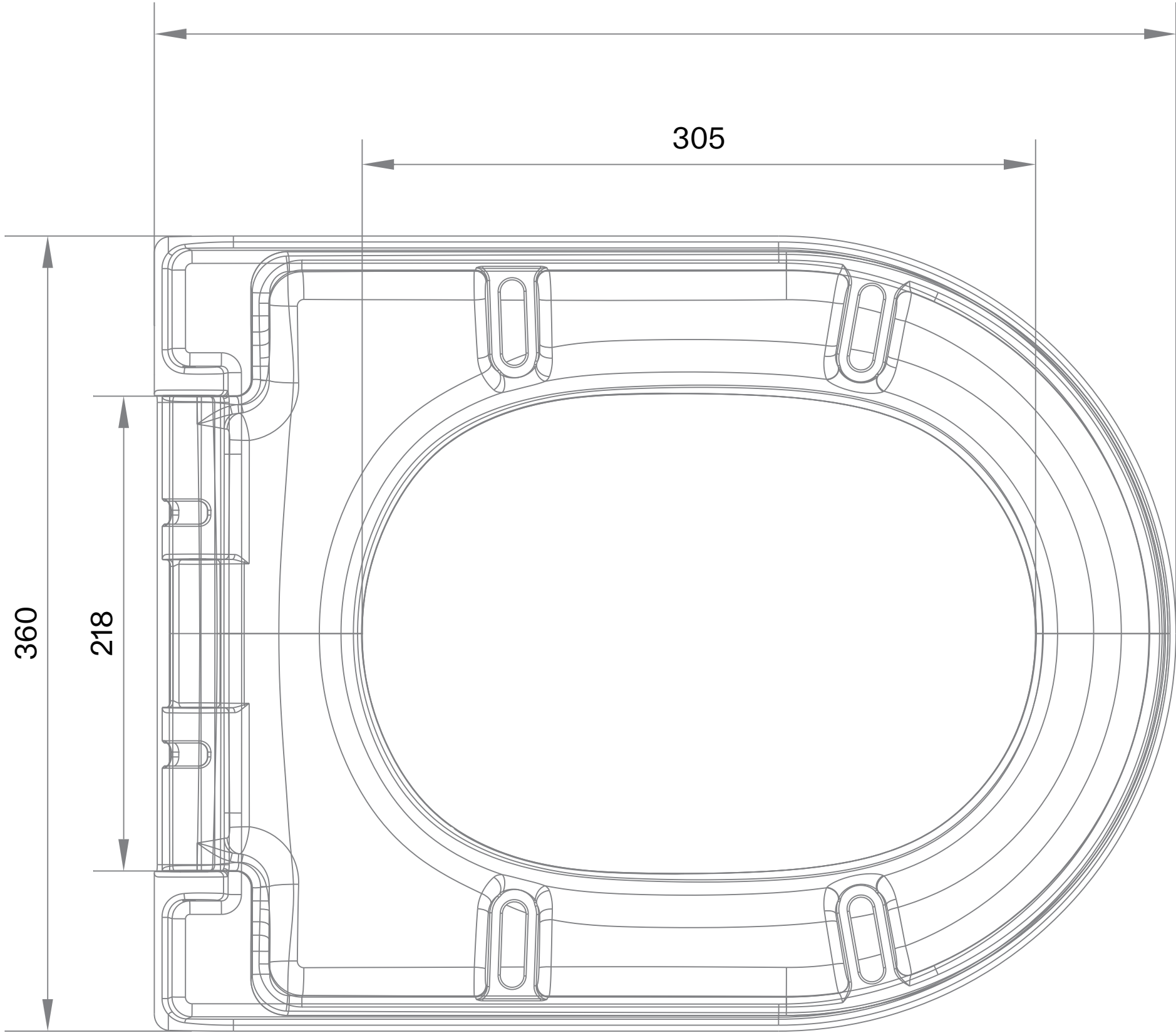
Bottom view
