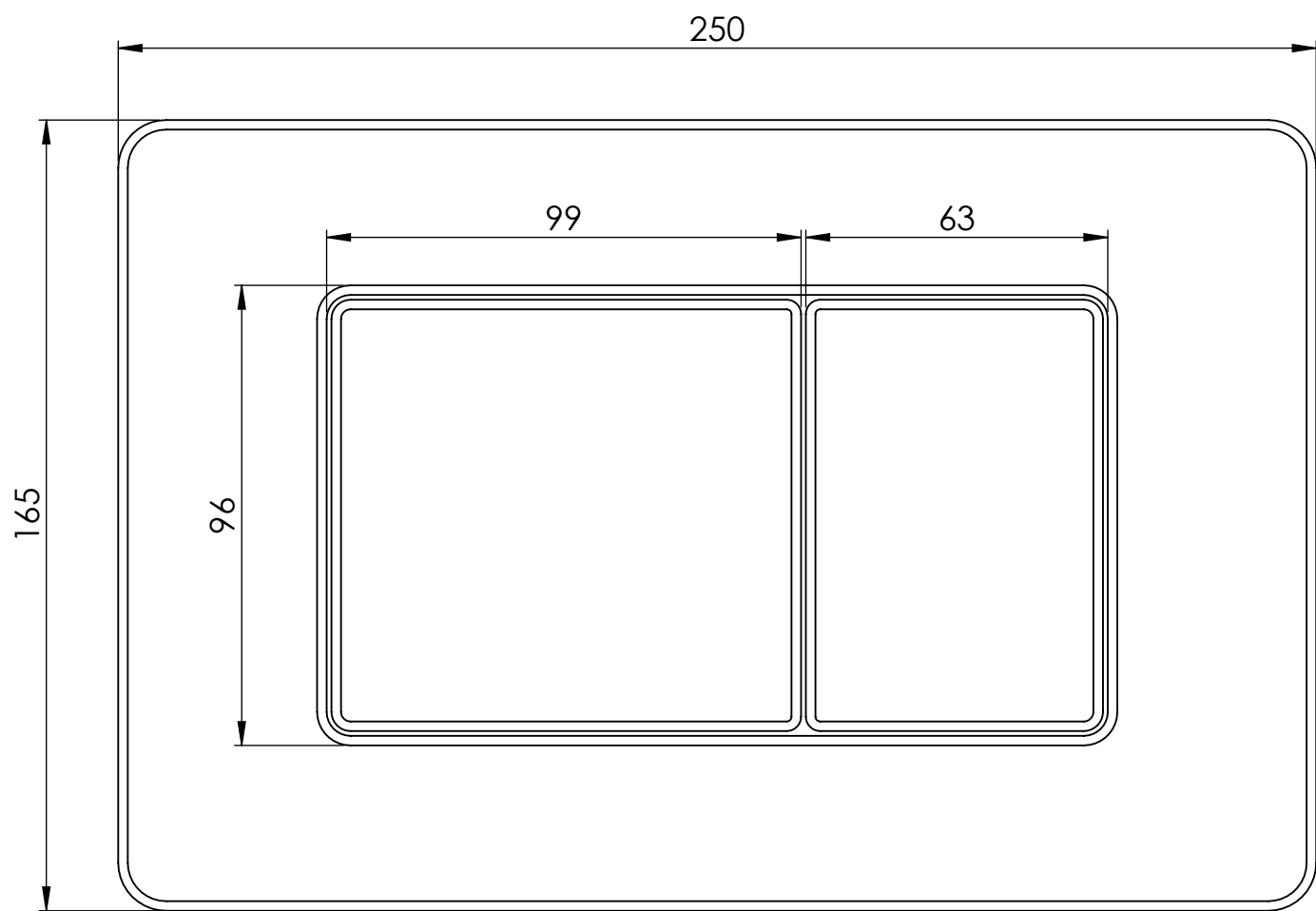
Front View
