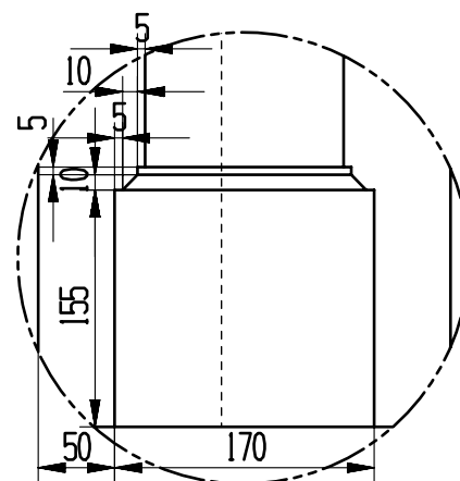
Detail C Scale 1:5
