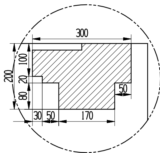
Detail B Scale 3:20
