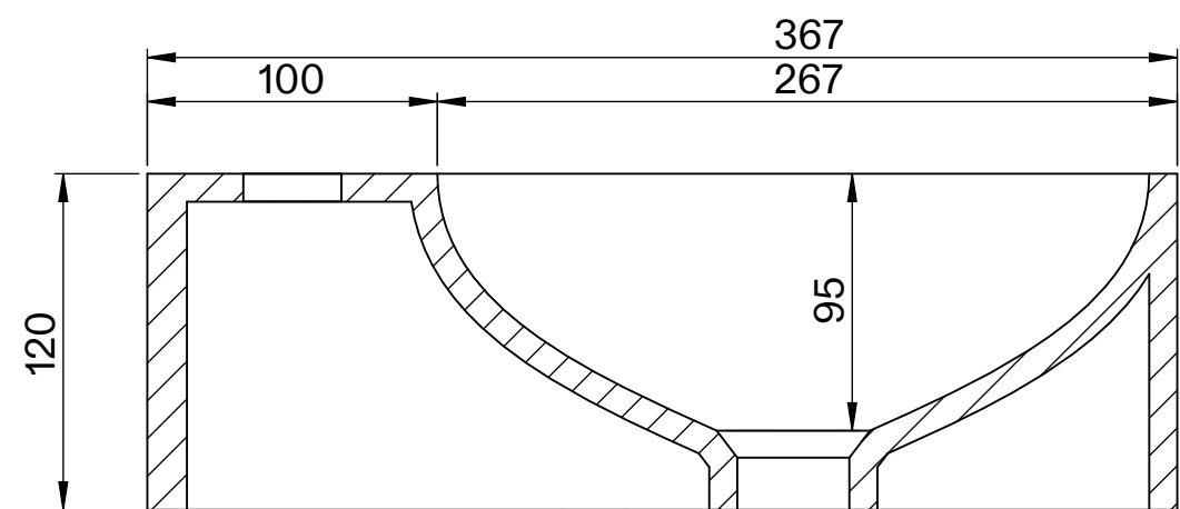
Section View
