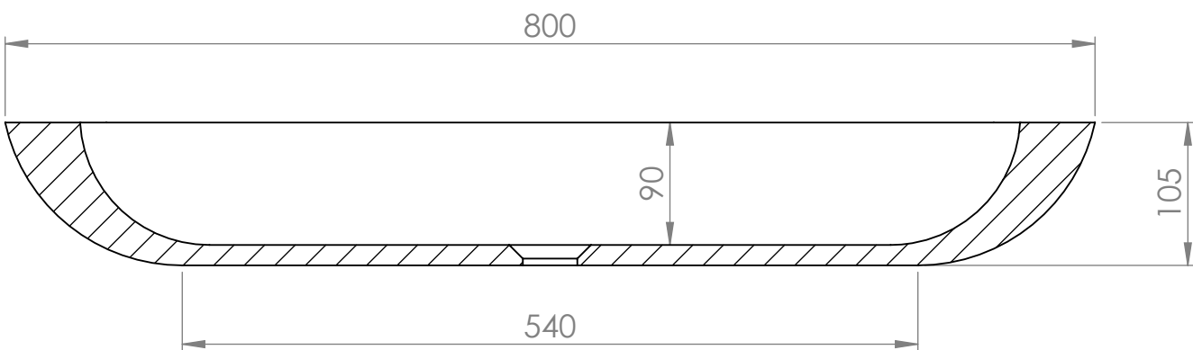
Side View - Section View
