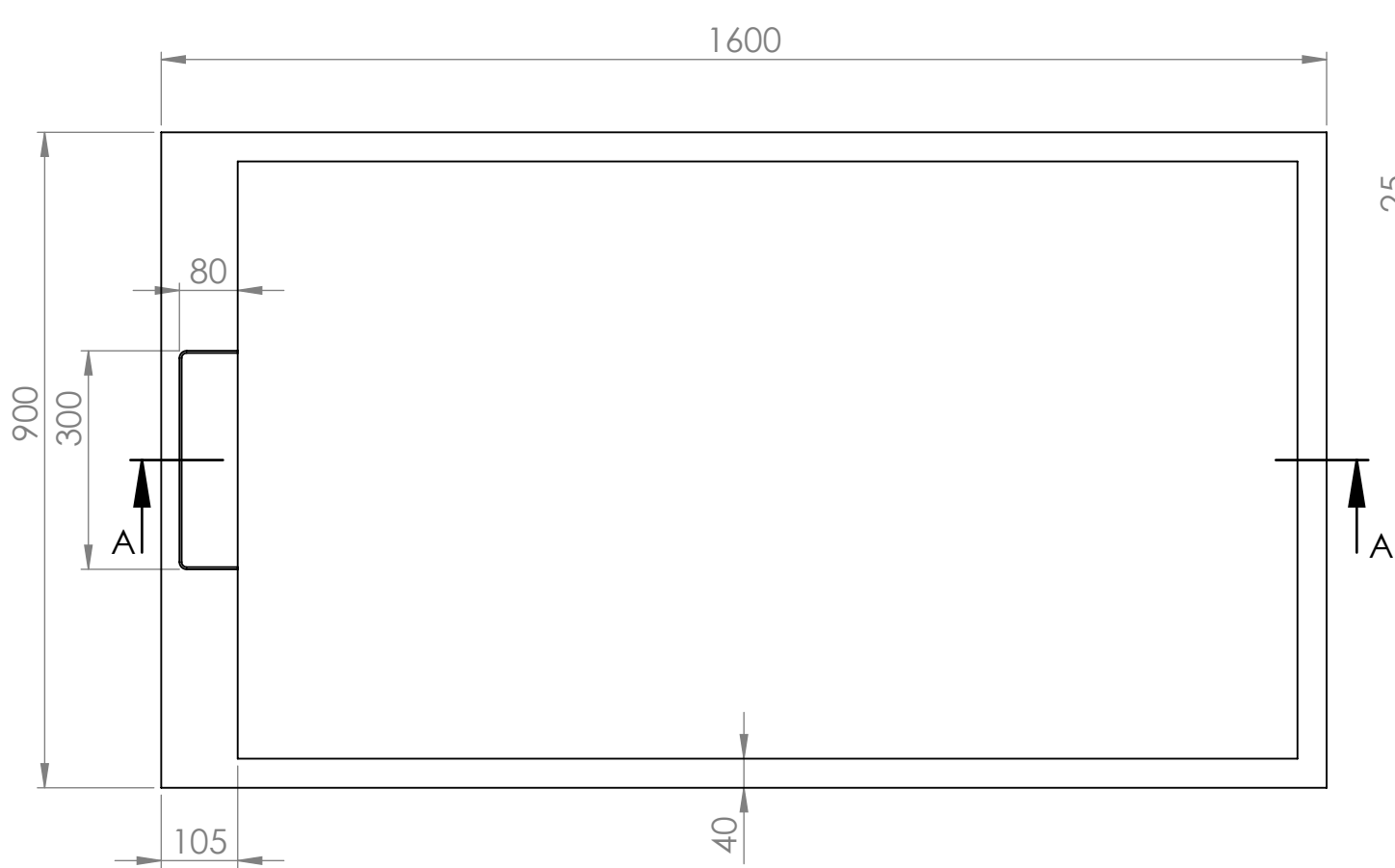
Shower Tray - Top View
