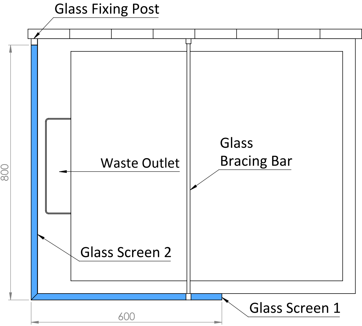
Shower Tray with Enclosure Kit - A
