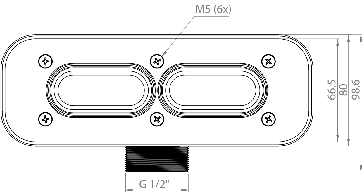
Waste Kit - Top View
