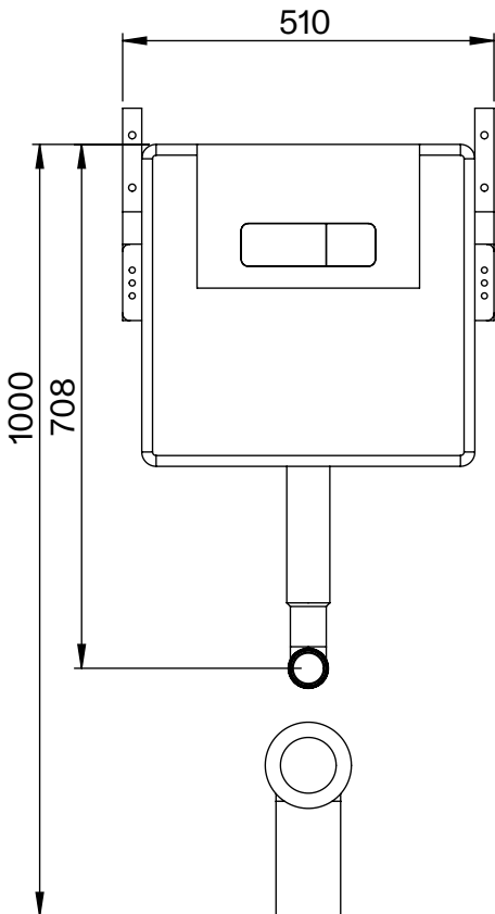
Front View
