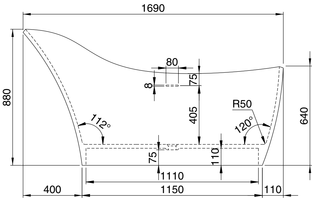
Front View - Section View
