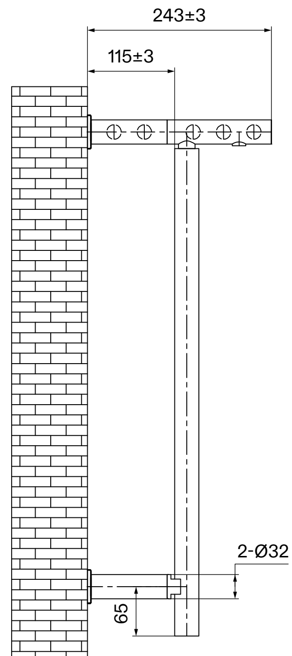
Side View
