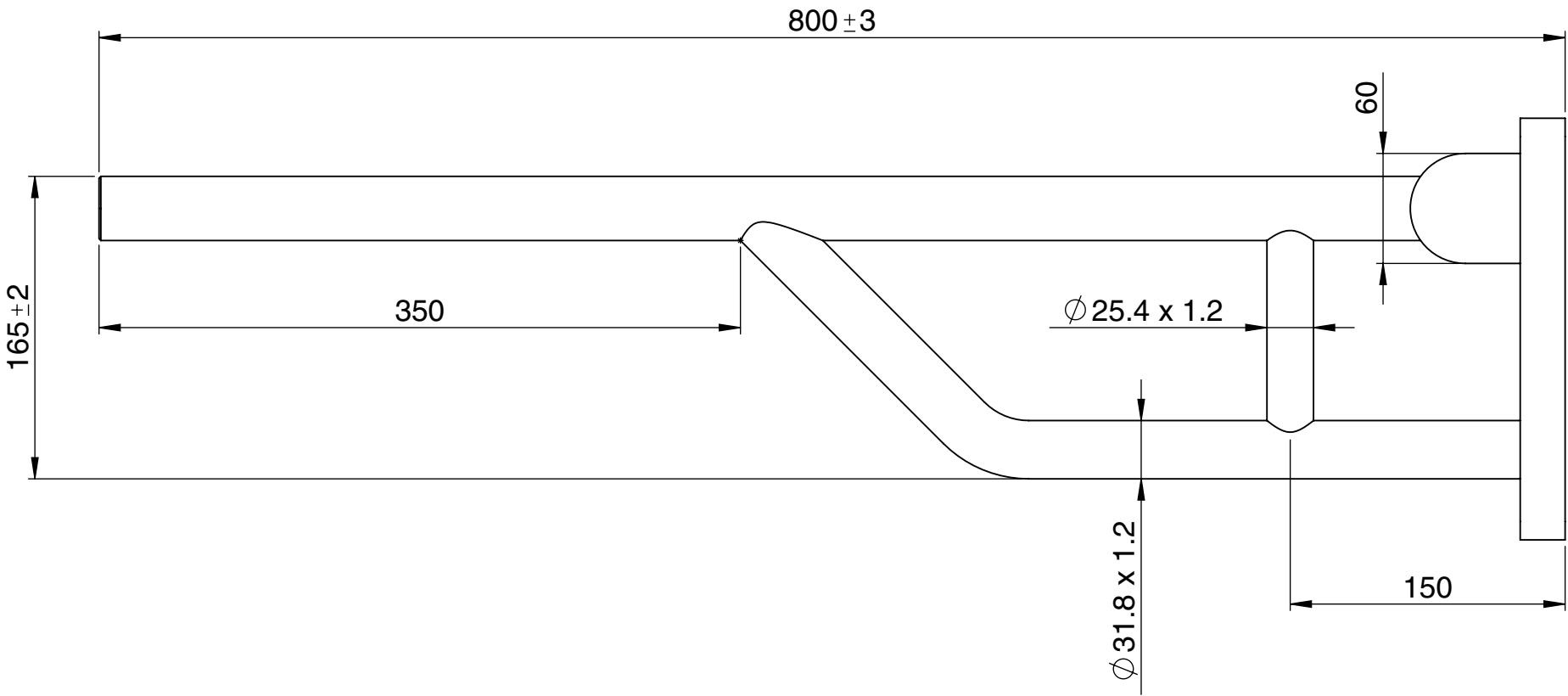
Front View
