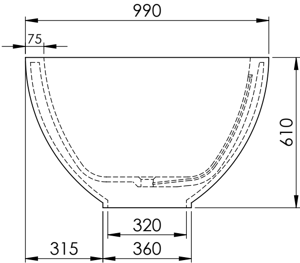
Side View - Section View
