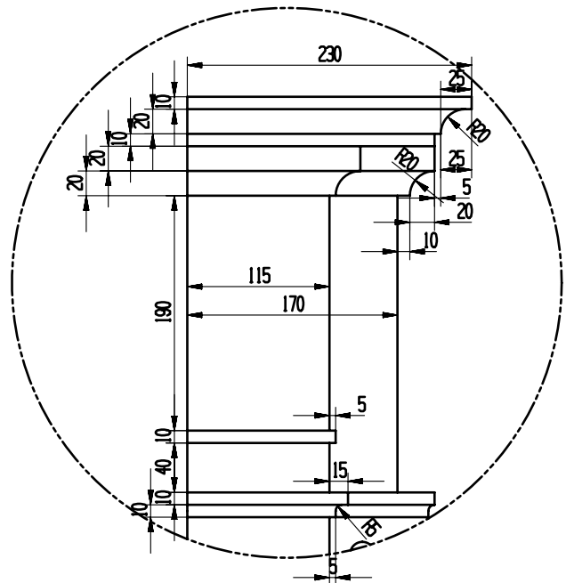
Section C Scale 3:10
