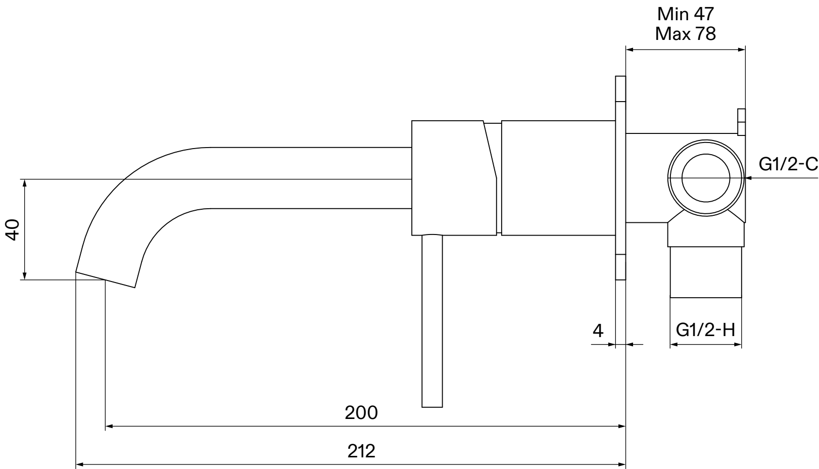
Side View
