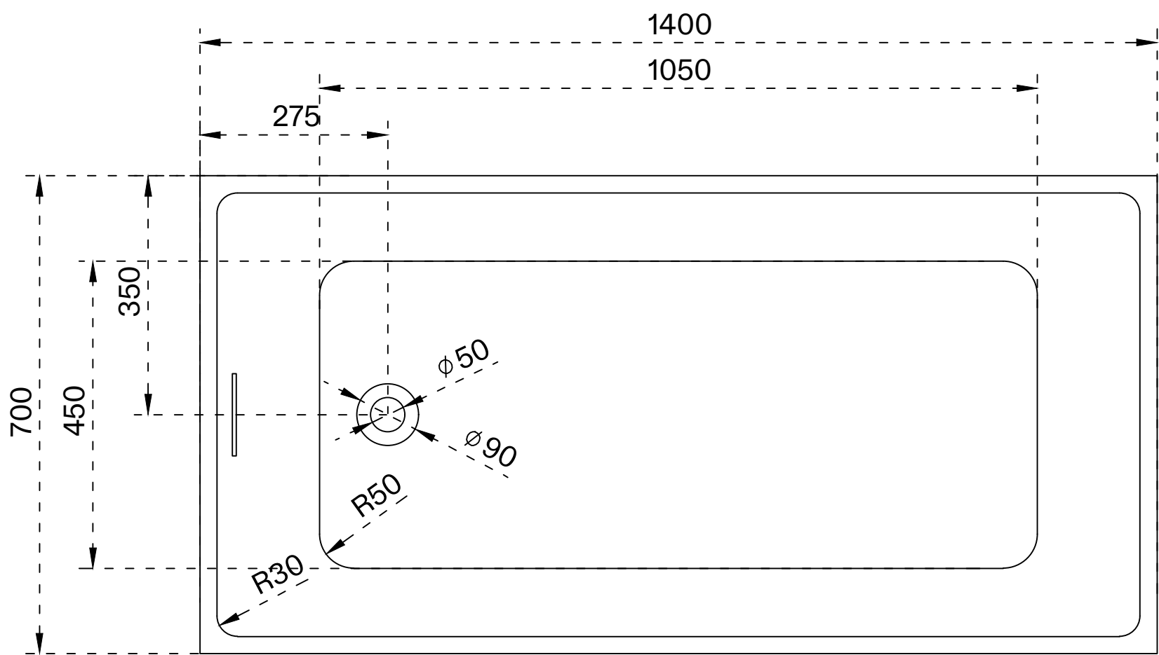
Top view
