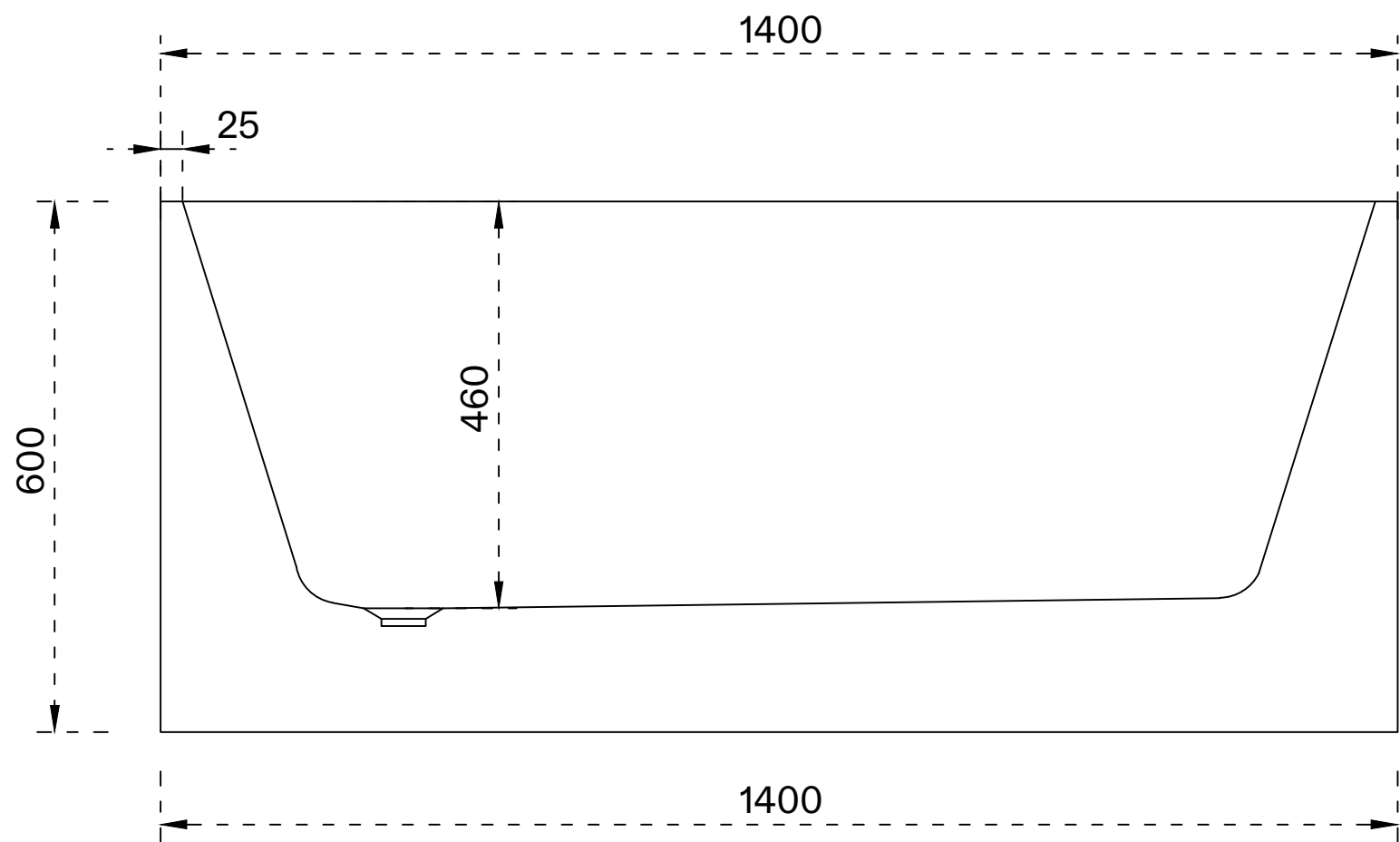
Side view
