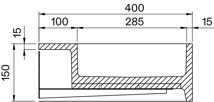
Side View - Section View
