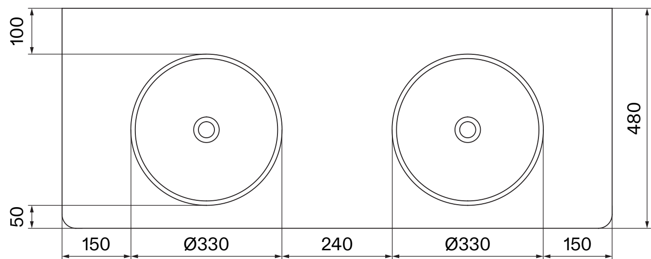
Top View
