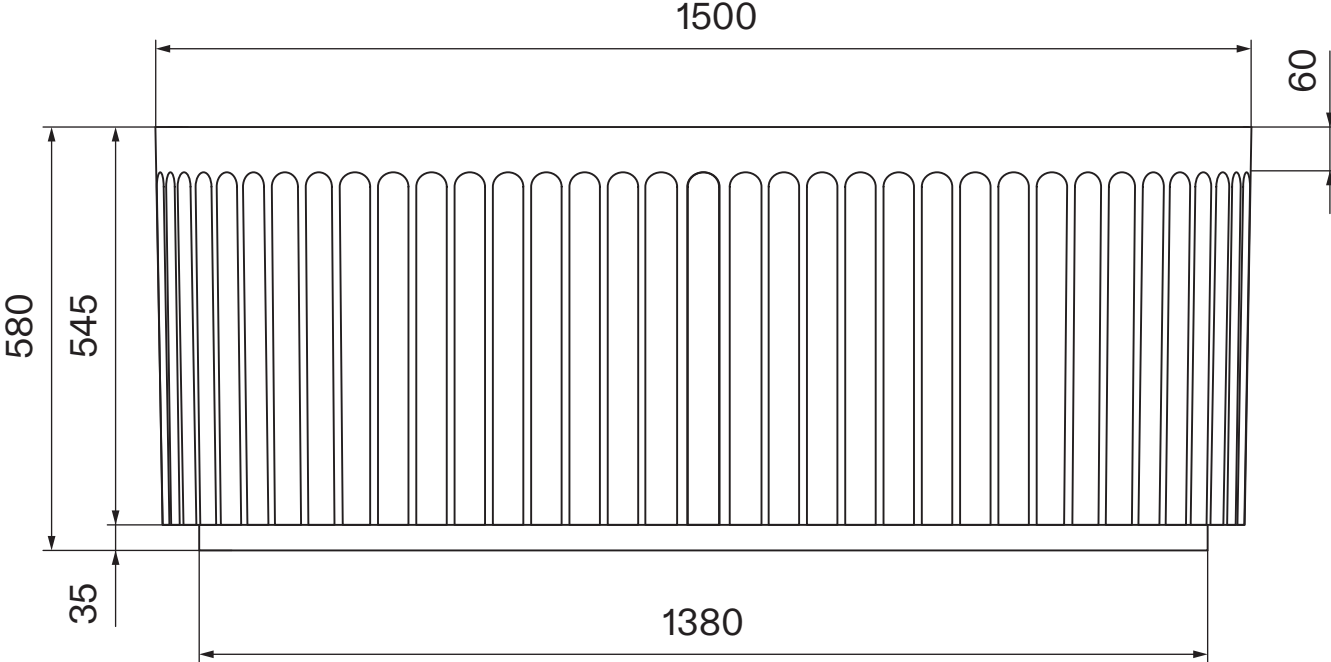
Detail A
