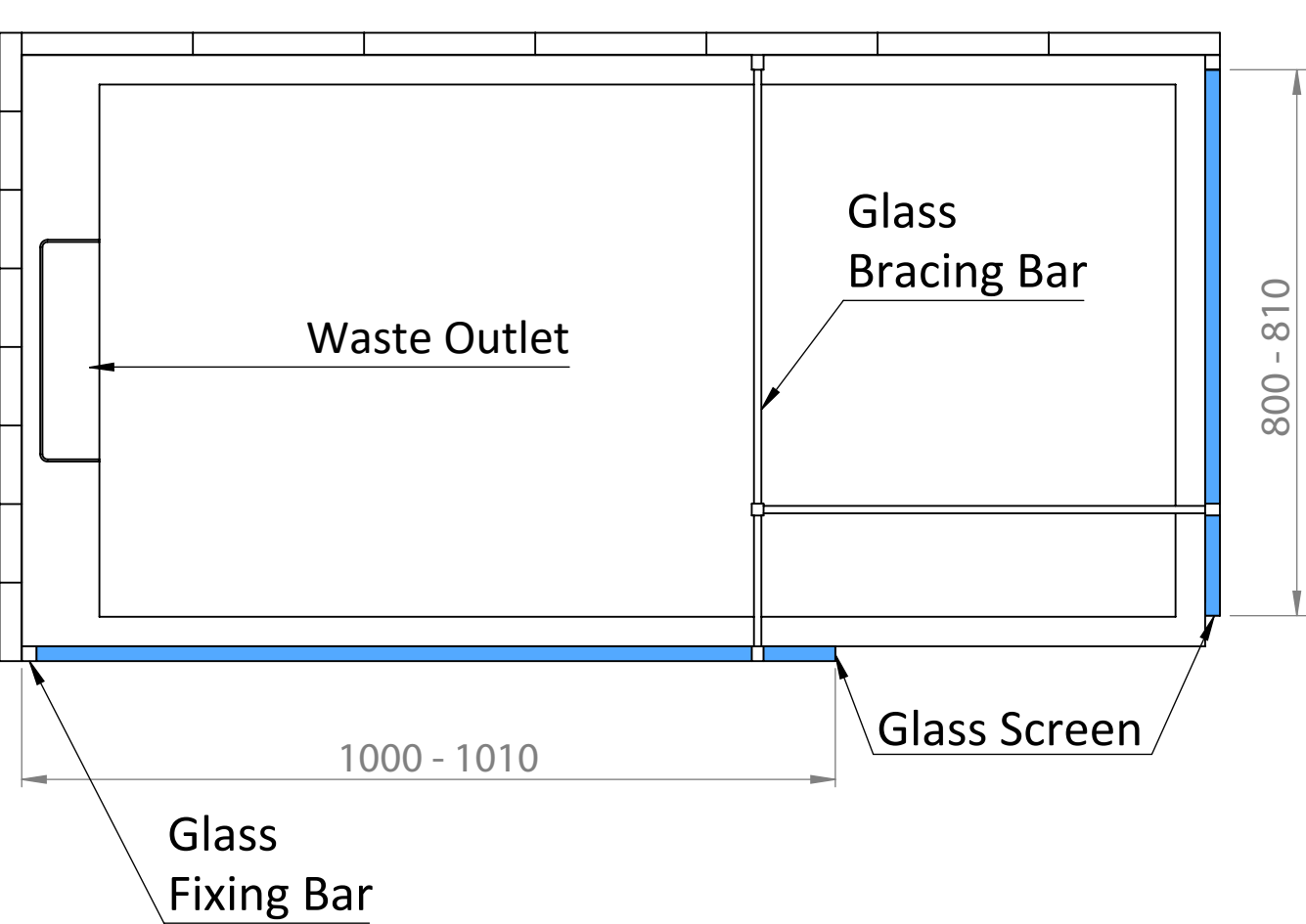
Shower Tray with Enclosure Kit - B
