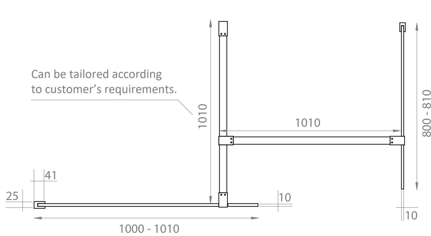
Top View
