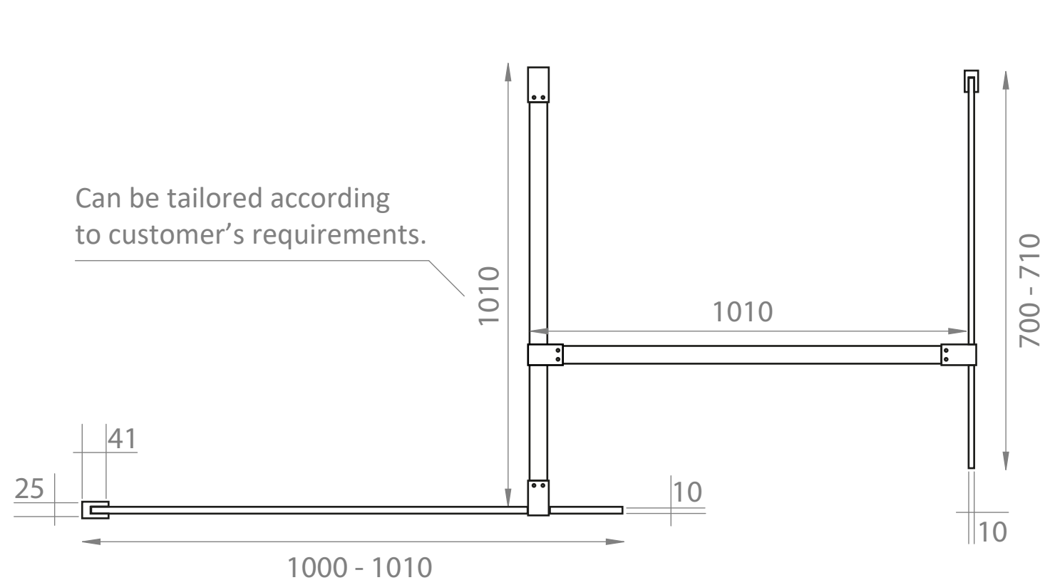
Top View
