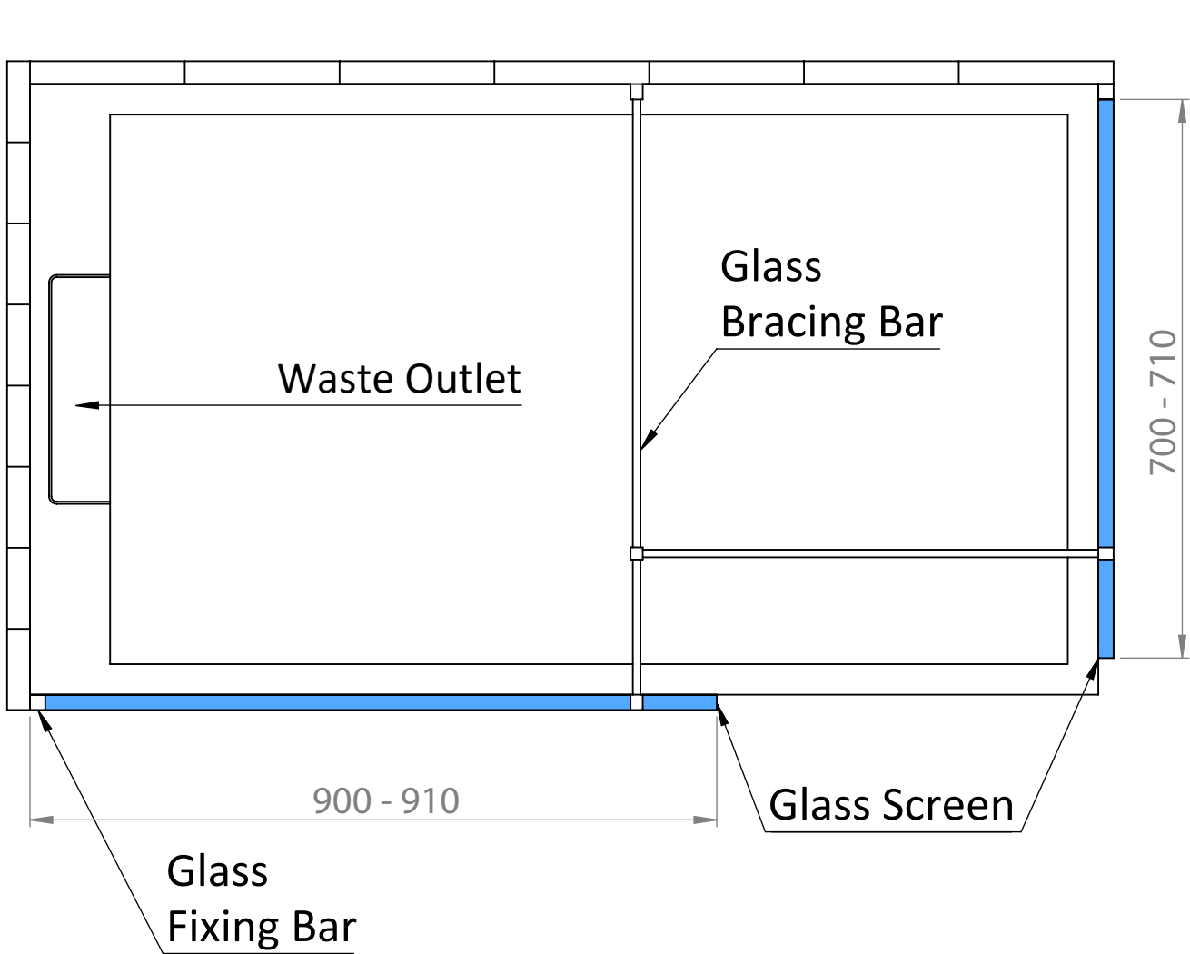
Shower Tray with Enclosure Kit - B
