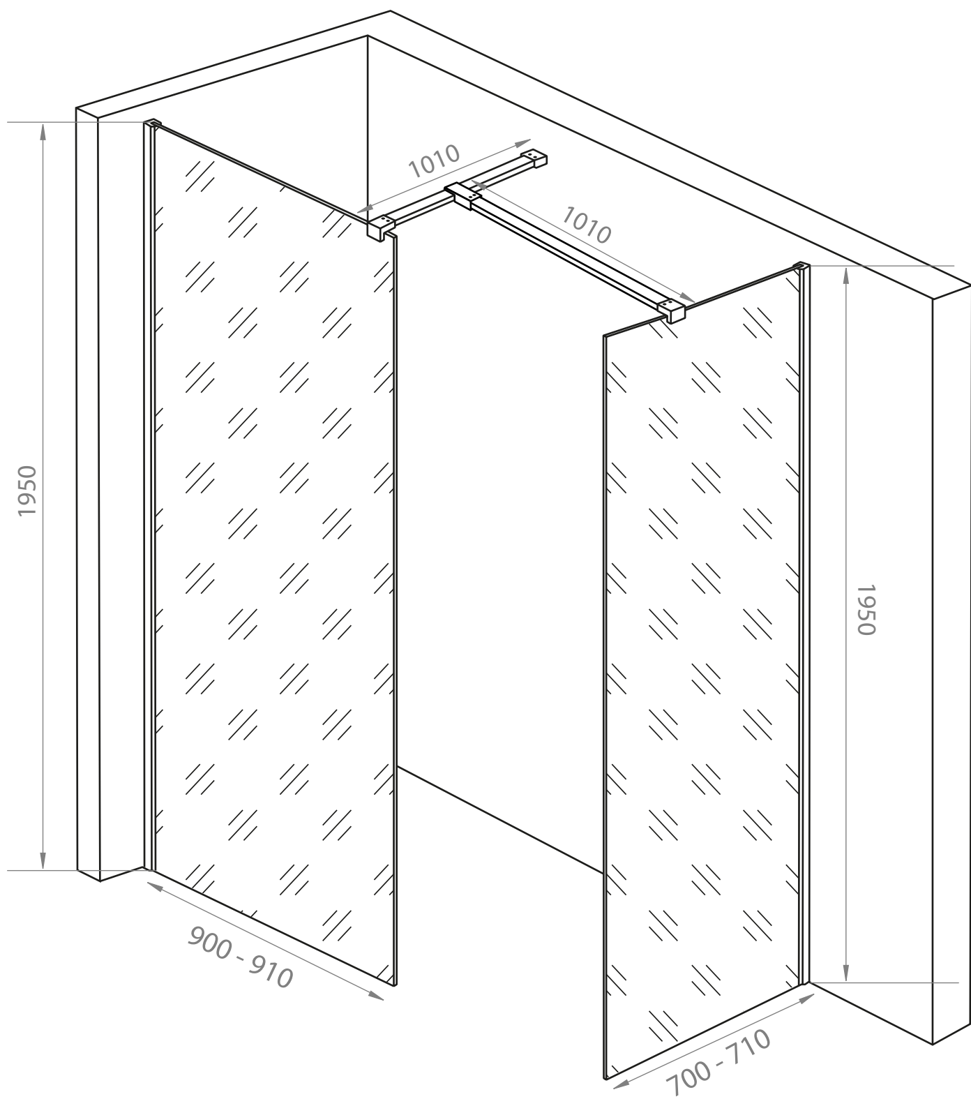
Full Enclosure View
