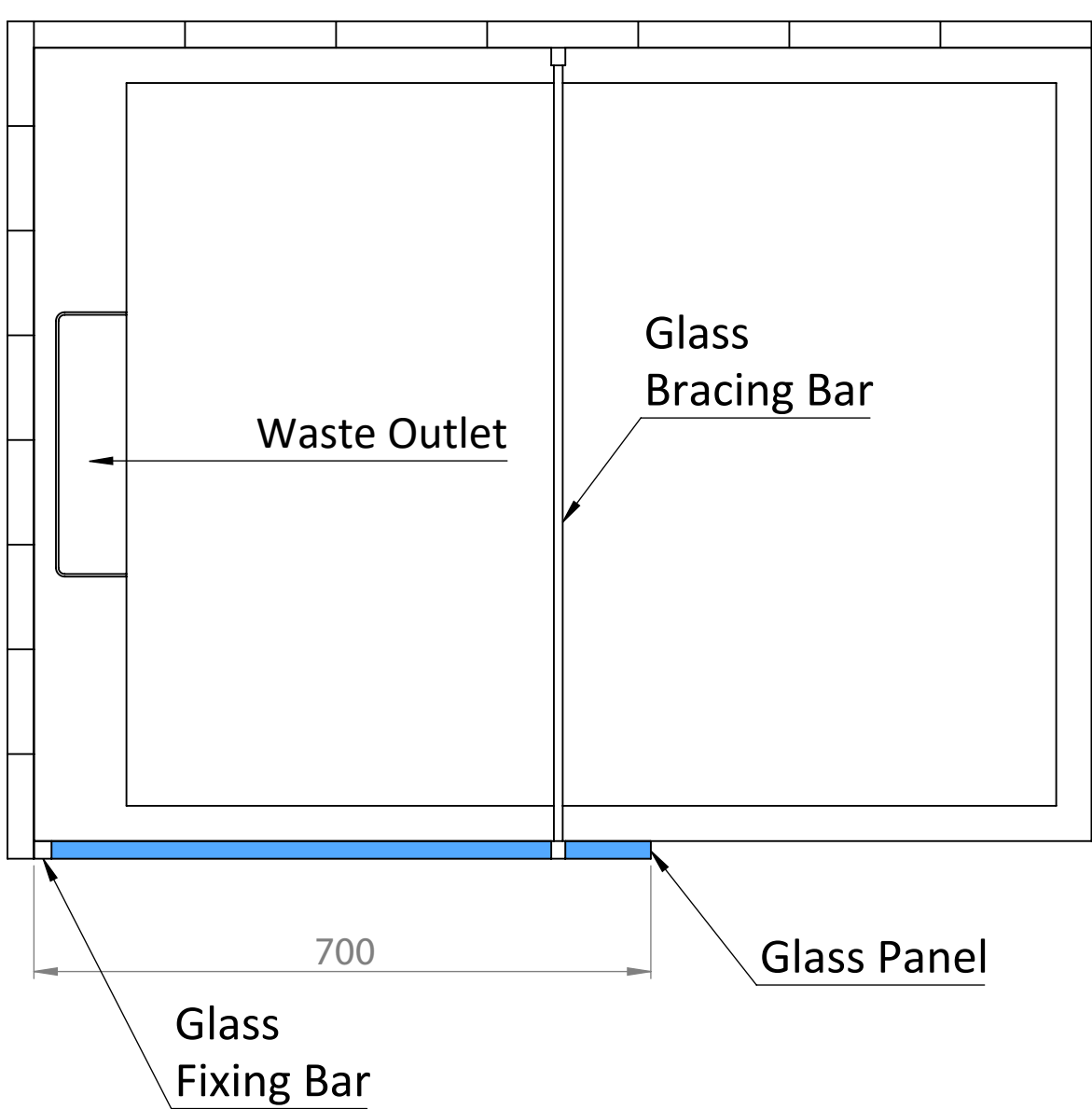
Shower Tray with Enclosure Kit - A
