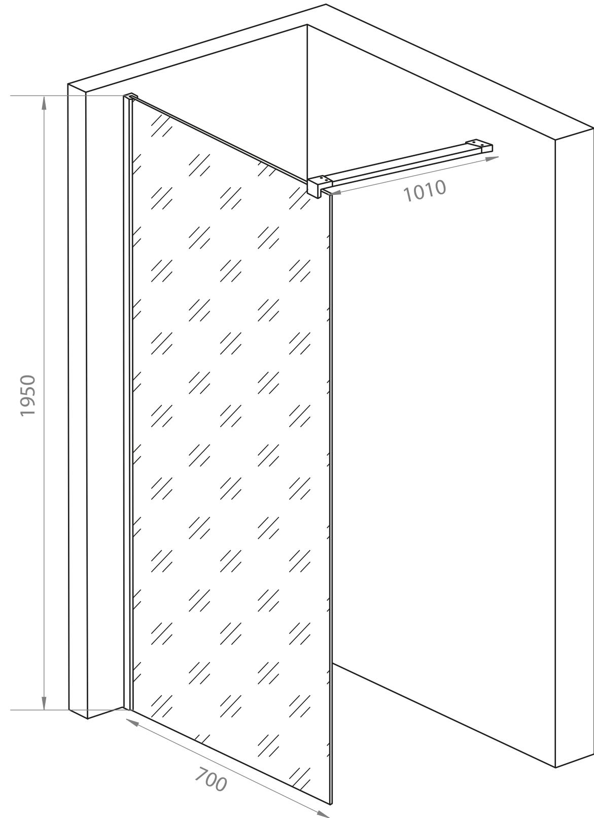
Full Enclosure View
