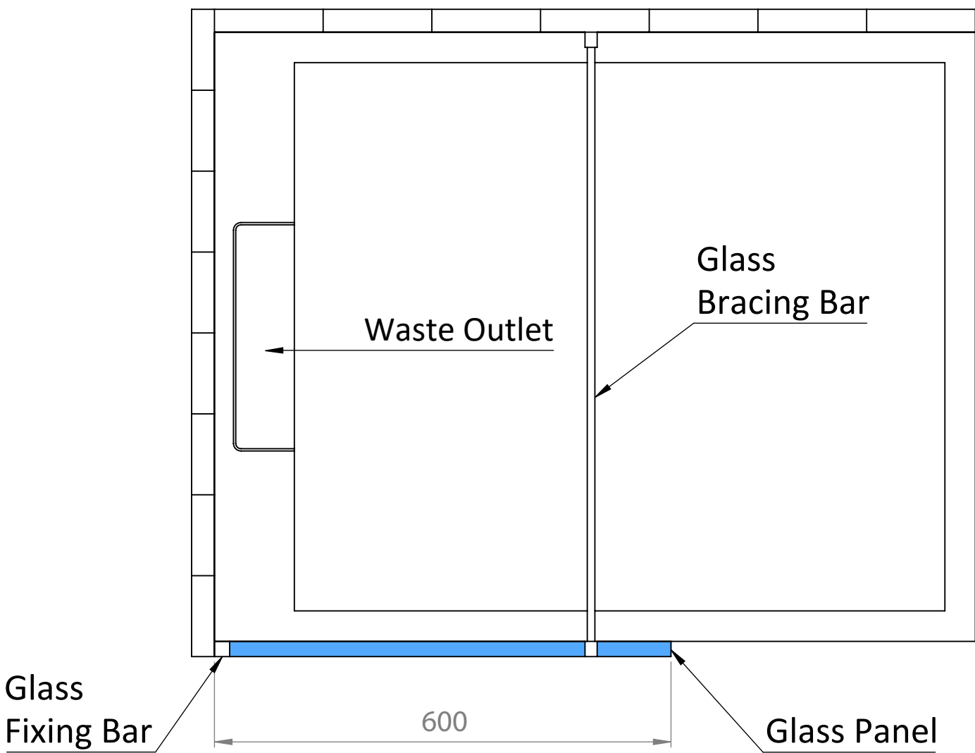
Shower Tray with Enclosure Kit - A
