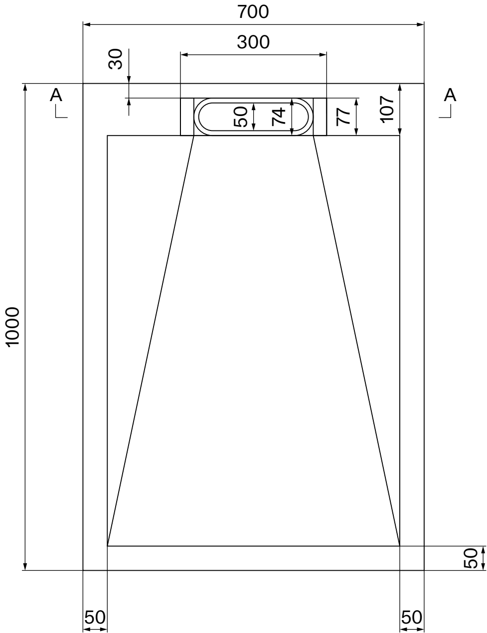
Top View
