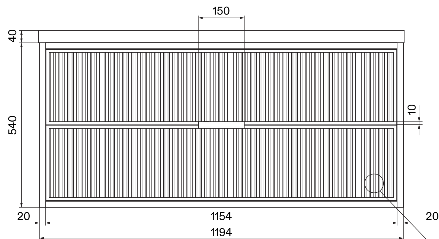
Front View - Vanity Unit
