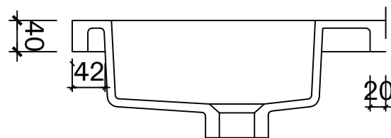
Side View - Basin
