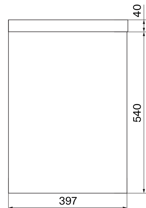
Side View - Vanity Unit
