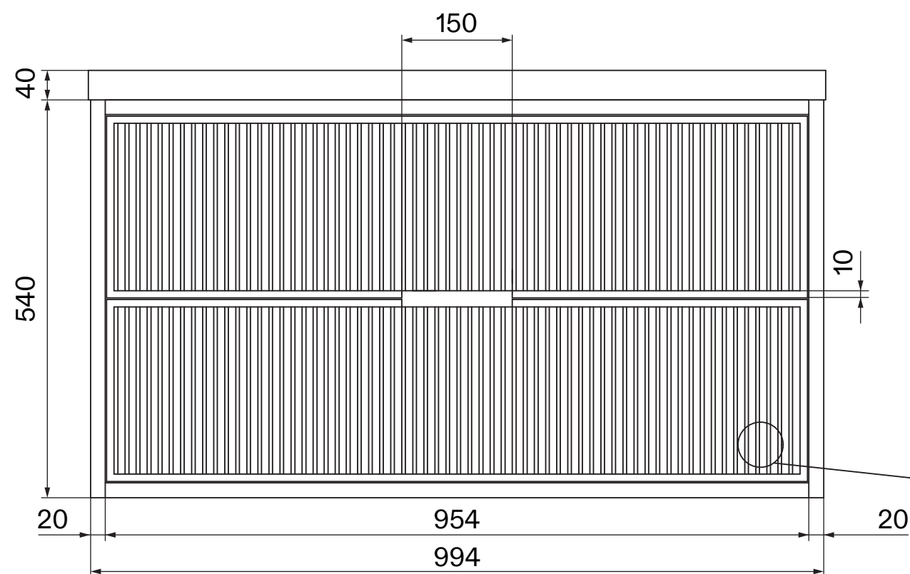
Front View - Vanity Unit
