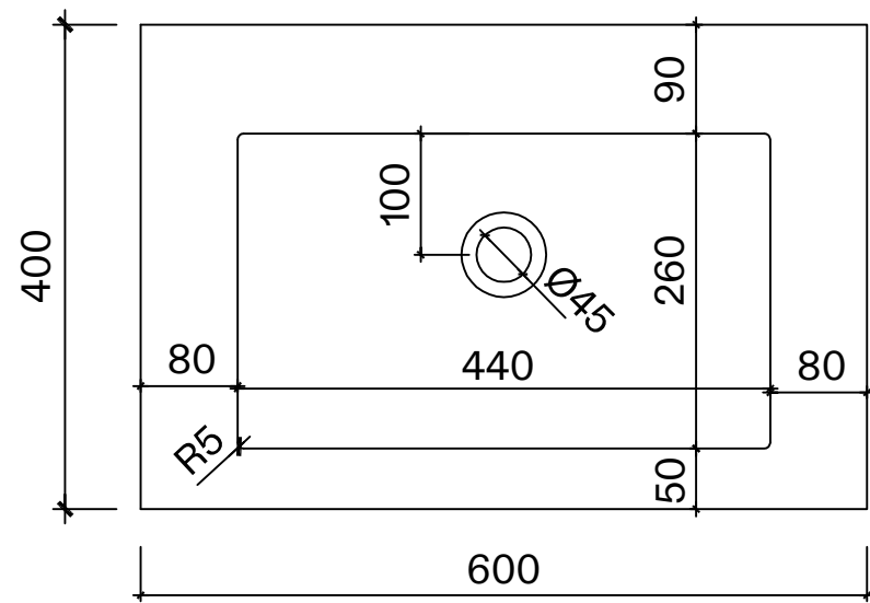
Front View - Basin
