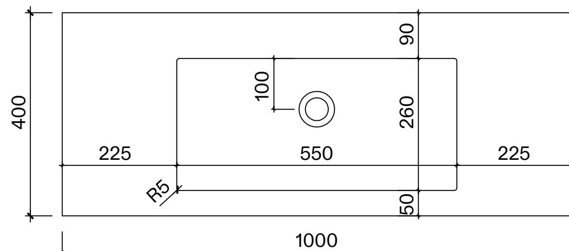
Front View - Basin
