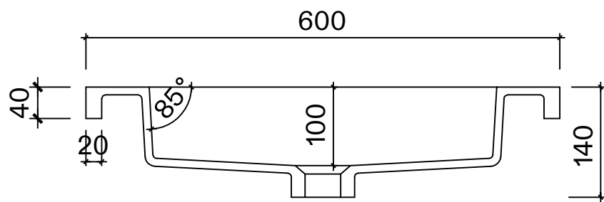
Front View - Basin
