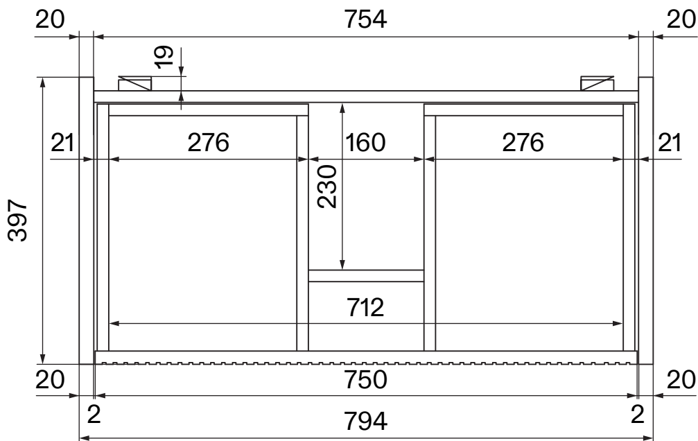
Bottom View - Vanity Unit
