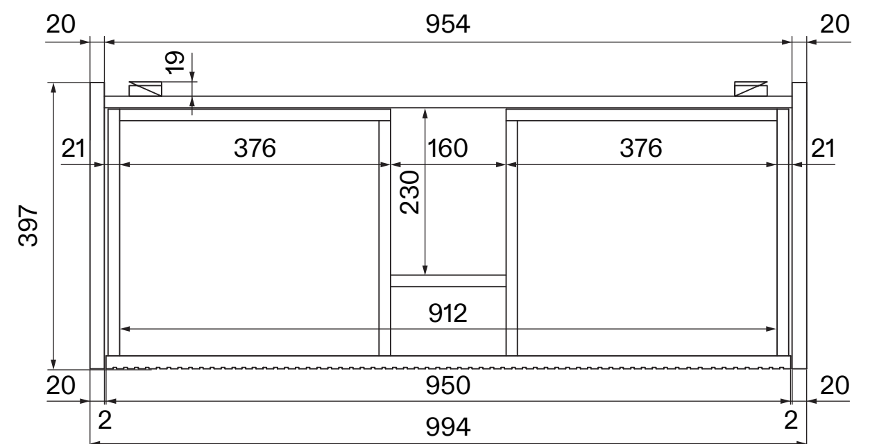
Bottom View - Vanity Unit
