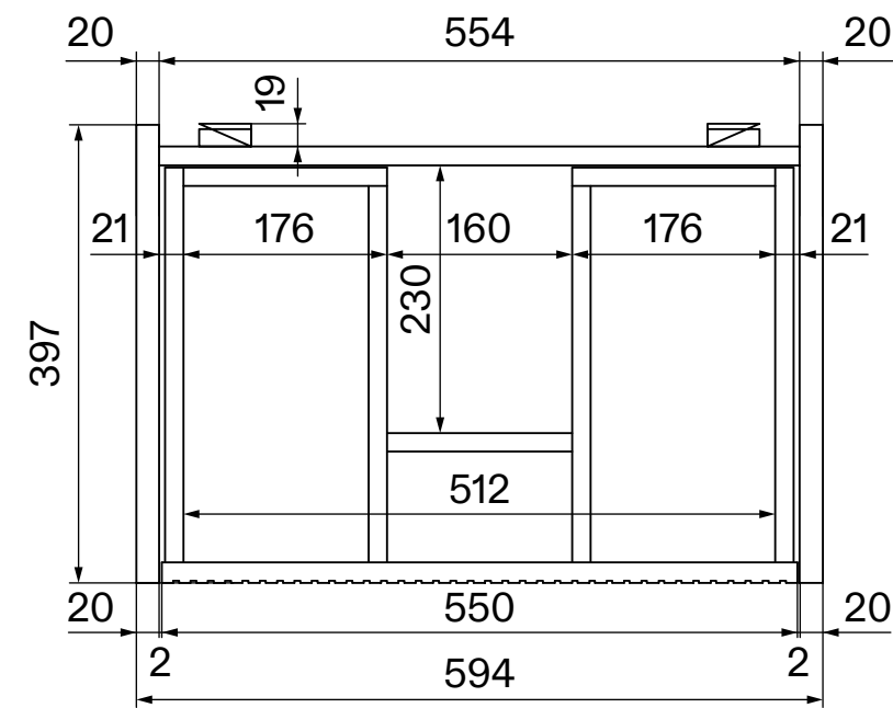
Bottom View - Vanity Unit
