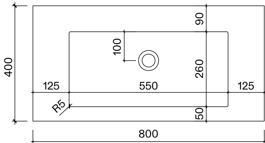
Top View - Basin
