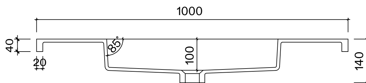
Top View - Basin
