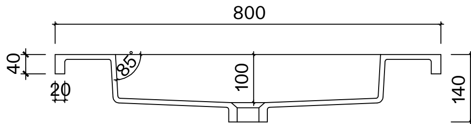
Front View - Basin
