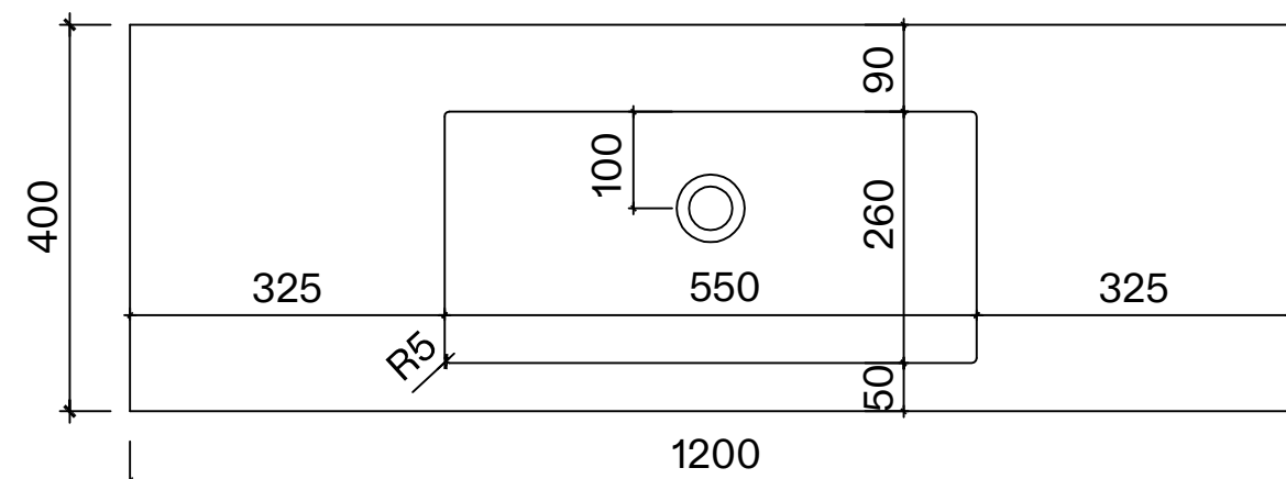
Top View - Basin
