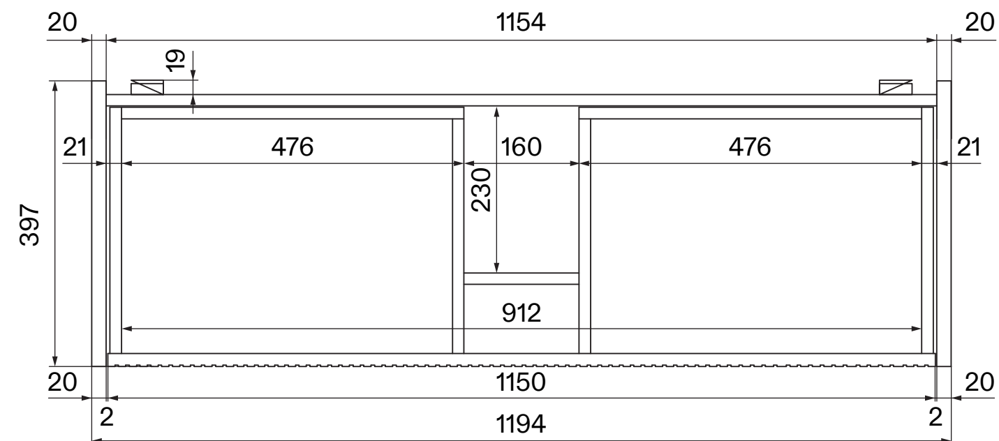
Bottom View - Vanity Unit
