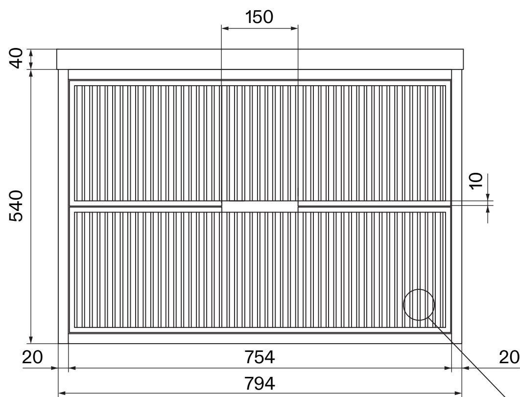
Front View - Vanity Unit
