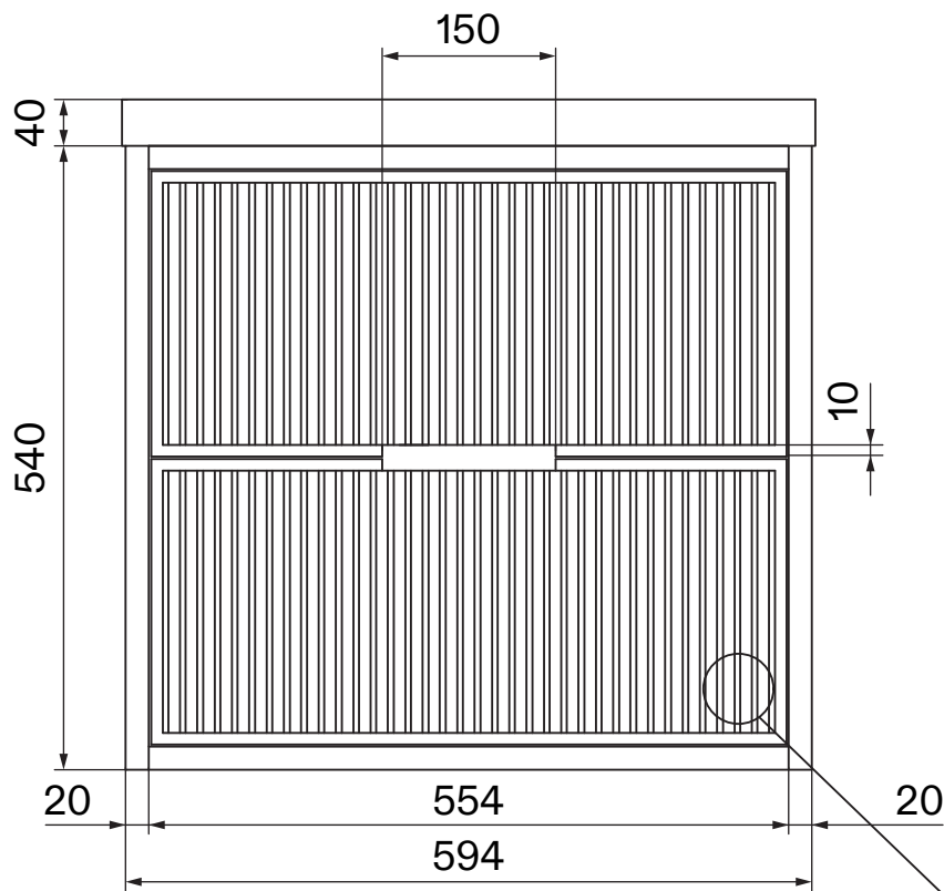
Front View - Vanity Unit
