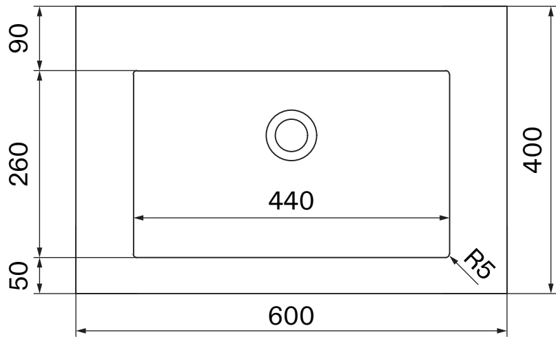
Bottom View - Vanity Unit
