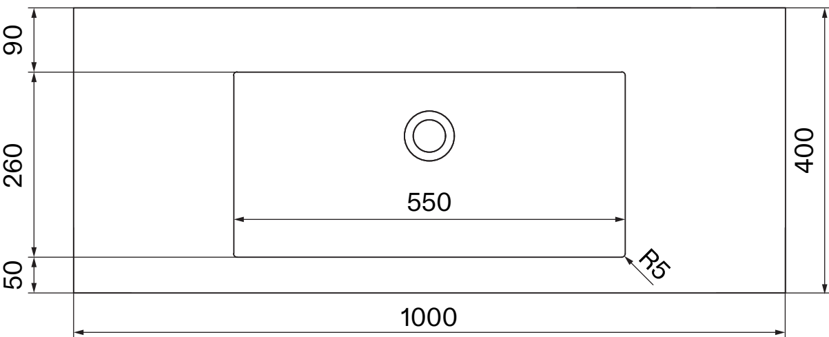
Bottom View - Vanity Unit
