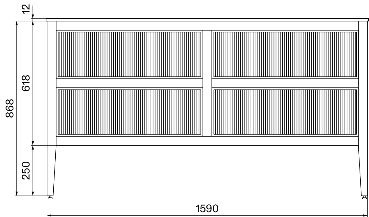
Front View
