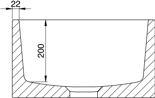
Side View - Section View
