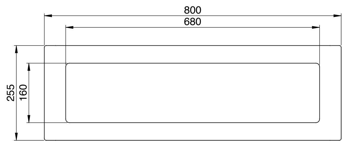
Front View
