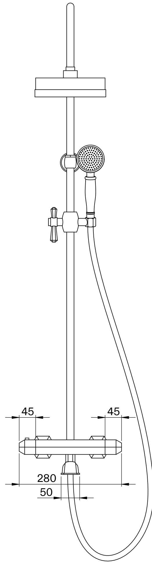
Front View
